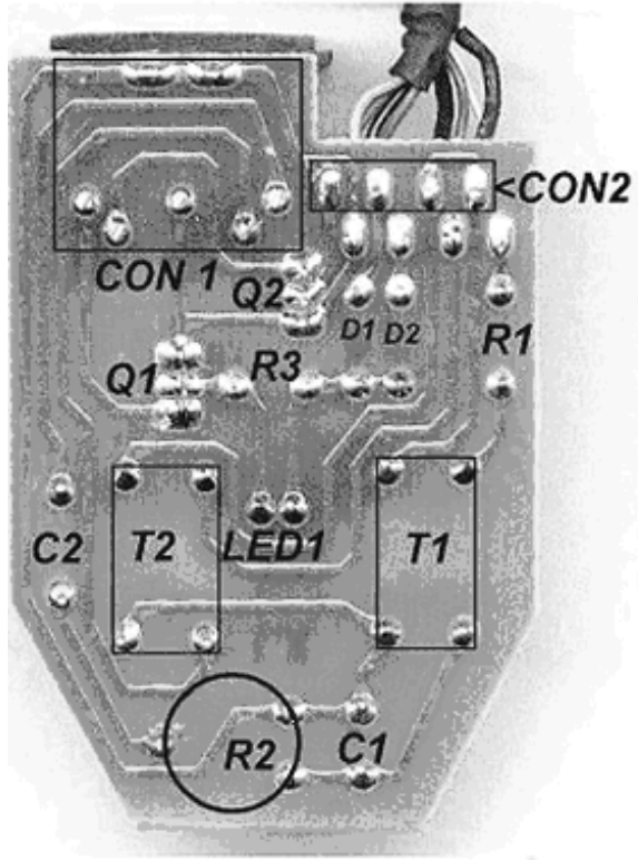
SOLDER SIDE OF PC BOARD
