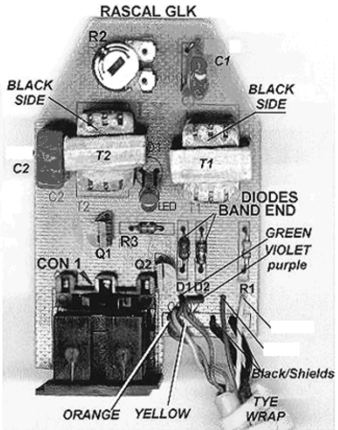
COMPONENT LAYOUT
