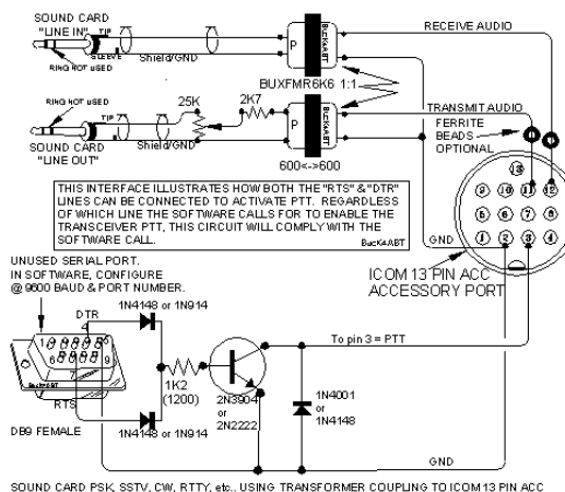
SOUND CARD PSK, SSTV, CW, RTTY, etc. USING TRANSFORMER COUPLING TO ICOM 13 PIN ACC
