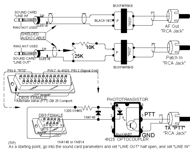
YAESU FT-757 and FT-767 rear panel RCA jacks to PC Sound Card for PSK31 mode.
