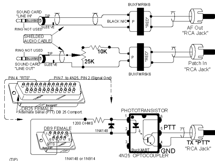
YAESU FT-757 and FT-767 rear panel RCA jacks to PC Sound Card for PSK31 mode.
